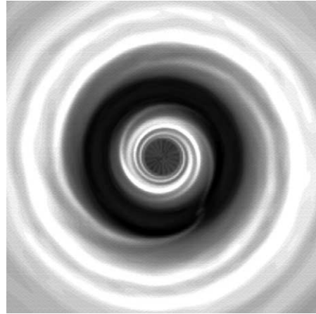
Fig. 1. A representative numerical simulation of a Jupiter-mass planet forming within a proto-planetary disk (from Bryden et al., 1999). White indicates high density while black indicates low density. The planet itself is within the gap (dark annulus), in a small accretion stream. While the planet itself is extremely difficult to detect at any wavelength, the wide gap is a strong marker of its presence. The SKA will have the resolution to resolve proto-planetary disks such as this one, detect the formation of planets, and even monitor the evolution of the disk.
