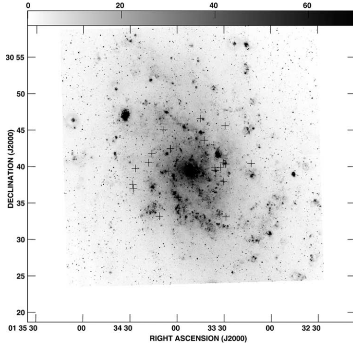
Fig. 3. Crosses mark the locations of young, dense H II regions found in a 2 h 5 GHz VLA A configuration observation overlaid on an H \alpha image of the nearest relatively face-on spiral M 33. From Pattison and Hoare, in preparation.
