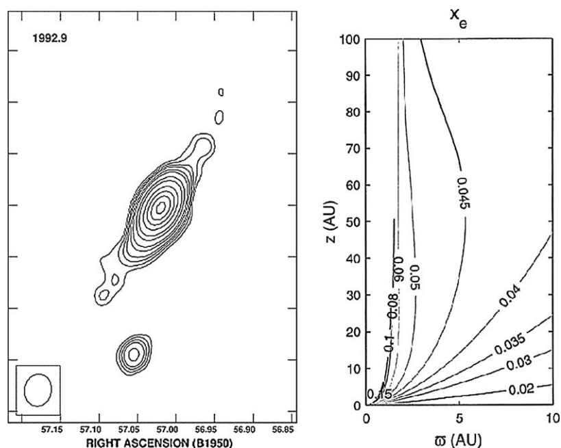
Fig. 1. (a) 6 cm VLA continuum map of the radio jet VLA 1 that powers the HH 1 region at 0.5'' resolution. The other unresolved source is VLA 2. The peak continuum brightness temperature is 100 K. From Rodríguez et al. (2000). (b) Predicted ionisation fraction structure for an X-wind model for YSO jets. Note the physical scale in AU assuming a distance of 150 pc appropriate for the nearest low-mass star-forming regions. From Shang et al. (2002).
